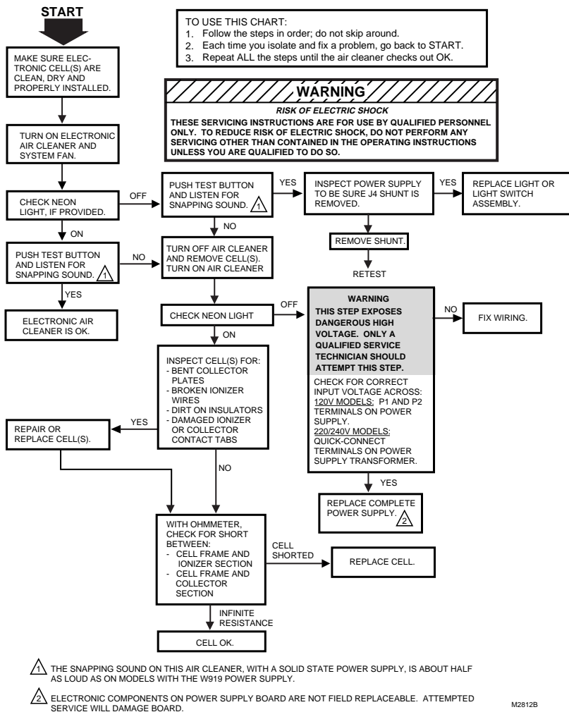
Fig. 19. Electrical troubleshooting procedure for electronic air cleaners in central systems.
